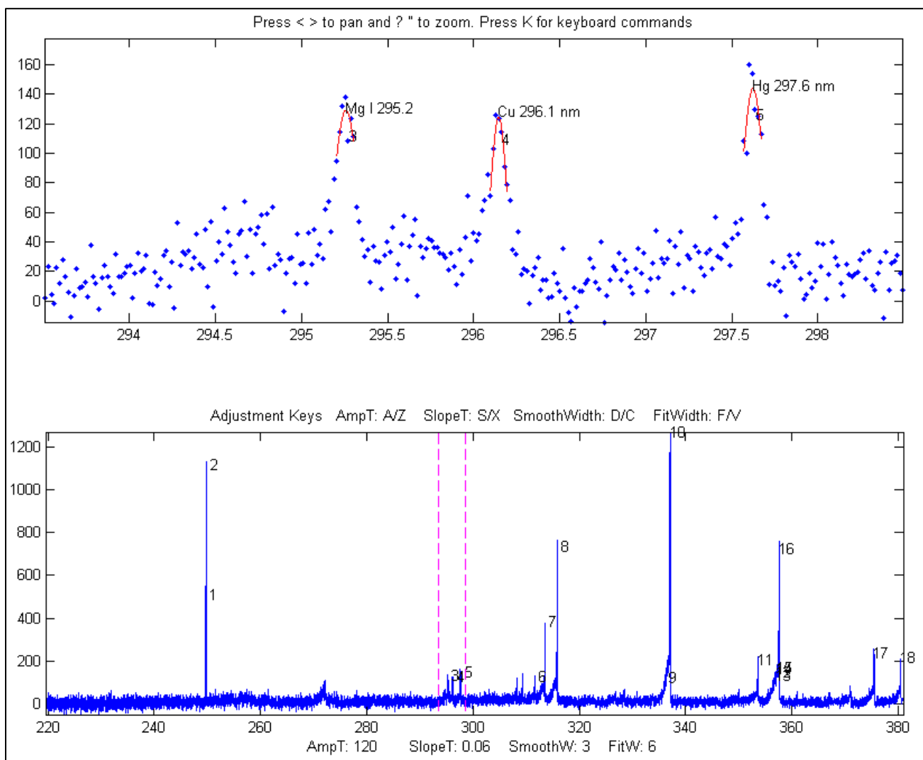
An atomic emission spectrum of a sample containing trace amounts of several elements. iPeak is used to zoom in to three small peaks near 296 nm. iPeak identified and labeled three peaks based on the atomic line data in ipeakdata.mat . Press the I key to display the peak ID names. Double-click the figure window title bar to expand to full screen for an even better view.
